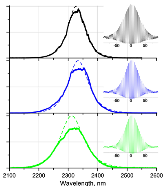
Fig. 23. Control of KLM laser parameters by translation of polycrystalline gain element along the waist of the laser beam. Emission spectra and the autocorrelation traces were measured for three different locations of the gain element (total translation along the waist within 0.5 mm). Dashed lines show the fit of measured spectra by sech profiles.
