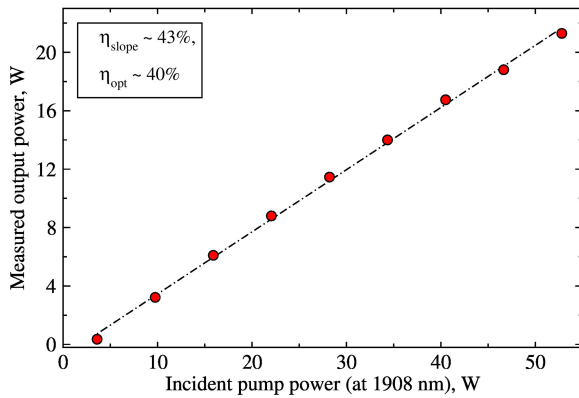
Fig. 4. Performance of \text{Cr}^{2+}:\text{ZnS} master oscillator at 2.4 \mu\text{m} pumped by a 50 W Tm fiber laser.
